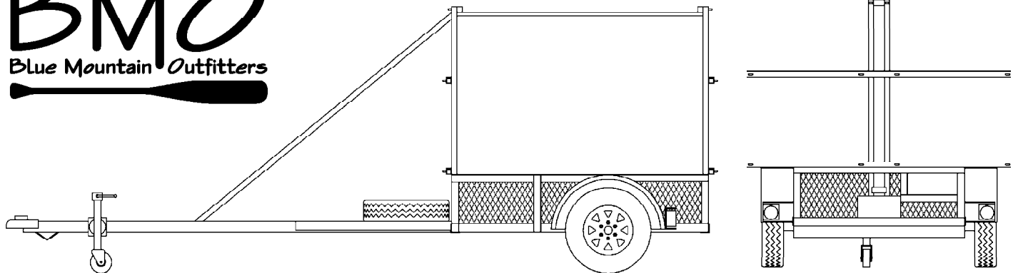
(4 boat trailer shown with optional stacker posts)
