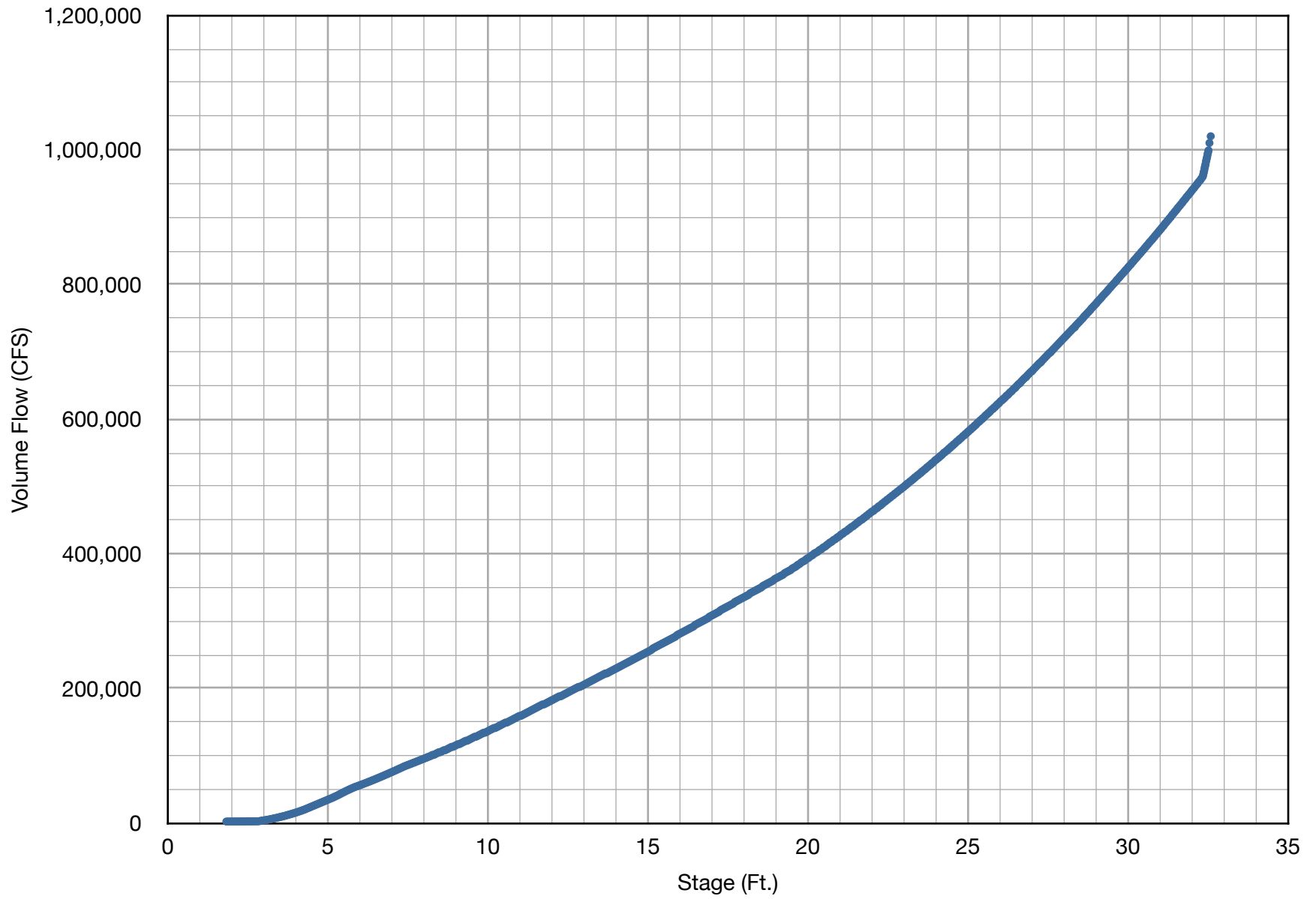
Susquehanna at Harrisburg - USGS Data Retrieved 2008-09-24
